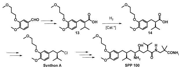
Scheme 2. Synthesis of Synthon A, a key intermediate in the preparation of the renin inhibitor SPP100.
