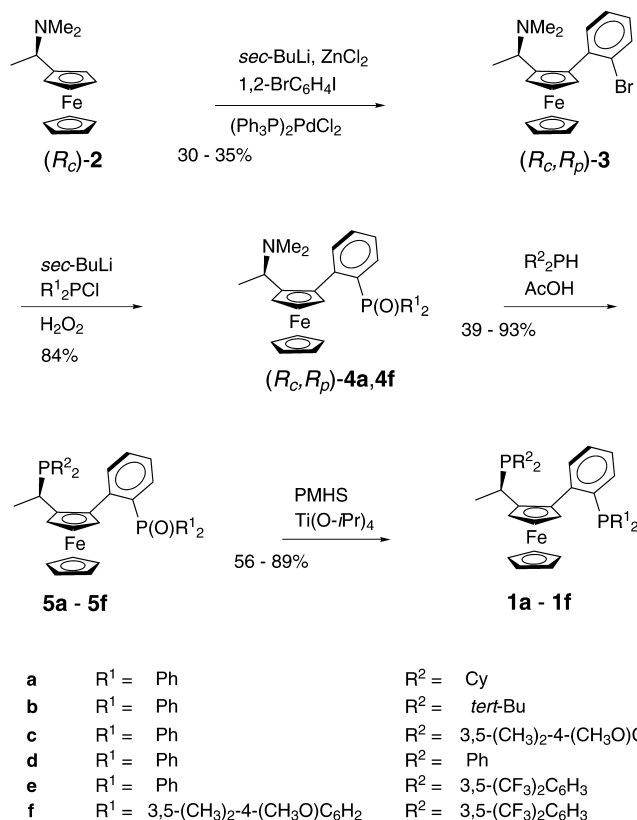
Scheme 1. Synthesis of ligands 1a–1f .
