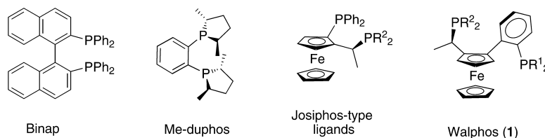
Figure 1. Examples of diphosphine ligands used in industrial enantioselective hydrogenation processes.
