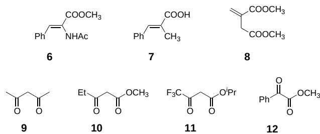
Figure 2. Olefins and ketones used as substrates in catalytic hydrogenations.
